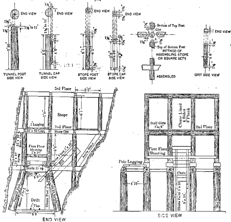
FIG. 3.—TIMBERING METHODS AT STEWARD MINE.
